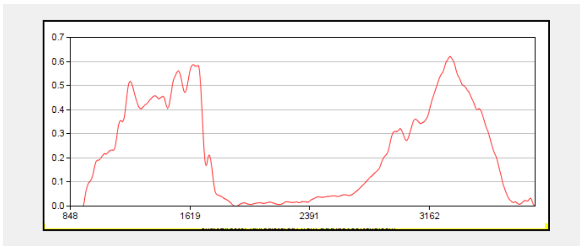
Figure 10: Reference Spectrum
