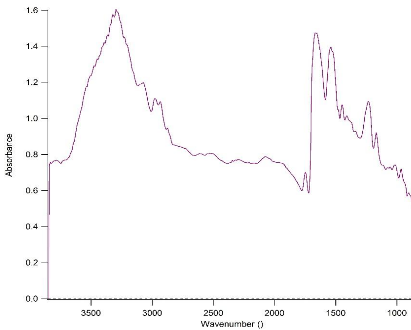
Figure 19: Average spectra of original image
